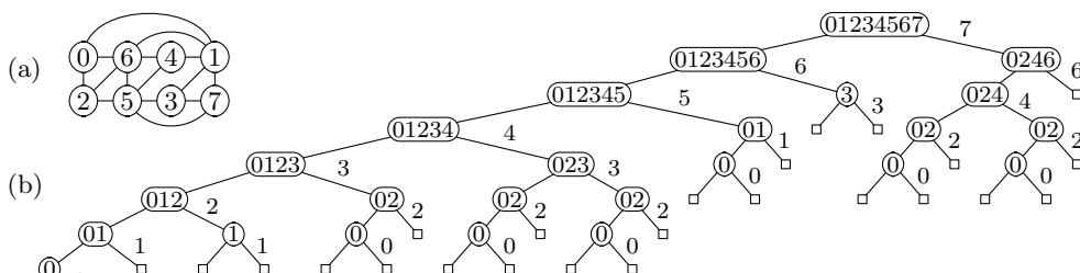
Fig. 400. A “random” graph, and a binary search tree for its independent sets.
